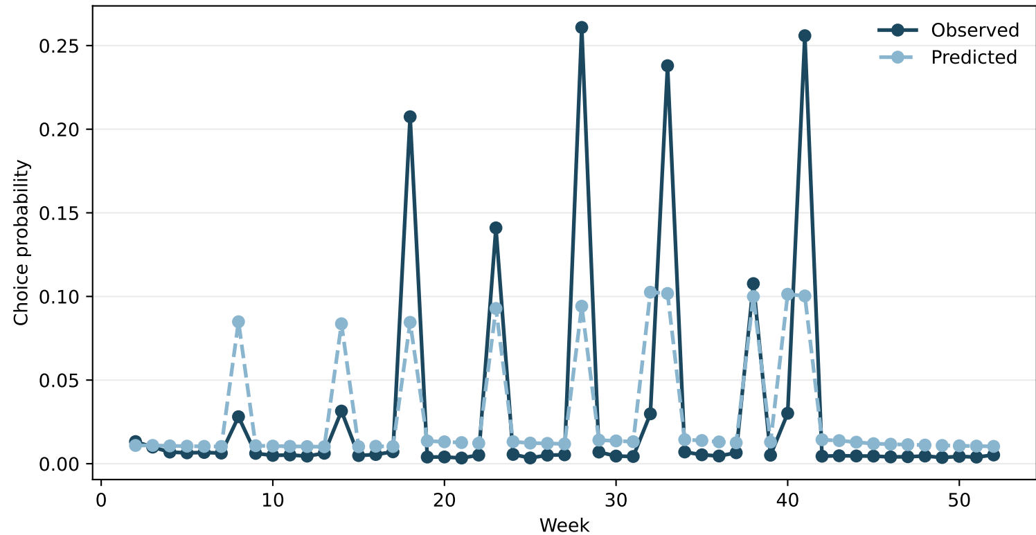
Observed vs. predicted choice probability: Glyngøre
